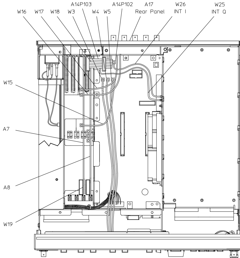
Option UN8/UN9 Top View
