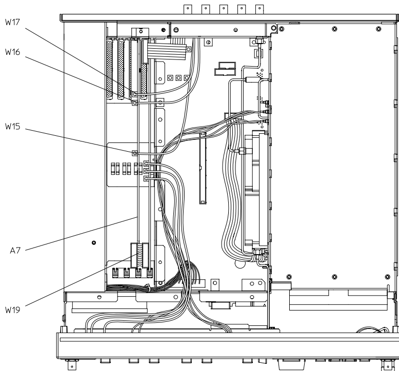
Figure 2 Option UN4 A7 Baseband Generator Board and Cables
