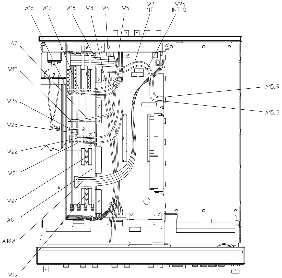
Figure 8 Options UN9/UN7/UND Top View
